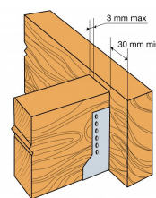
Installation on joist
