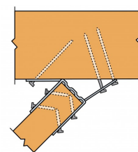
LSSU Installation
