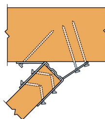
Sloped connection.
