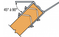
LSSU Installation
