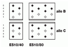
Nailing guide
