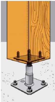
APB100/150 Installed
