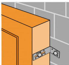
Timber to masonry connection
